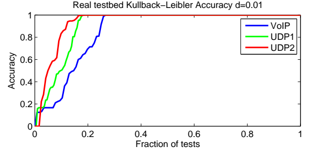
(a) Kullback-Leibler Divergence Accuracy
