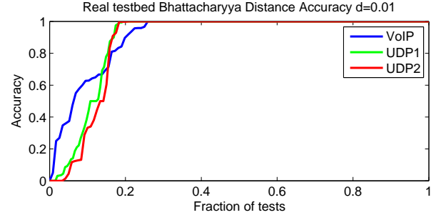
(b) Bhattacharyya Distance Accuracy
