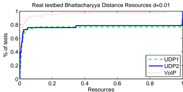
(b) Bhattacharyya Distance Resources
