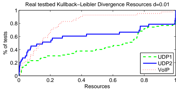
(a) Kullback-Leibler Divergence Resources
