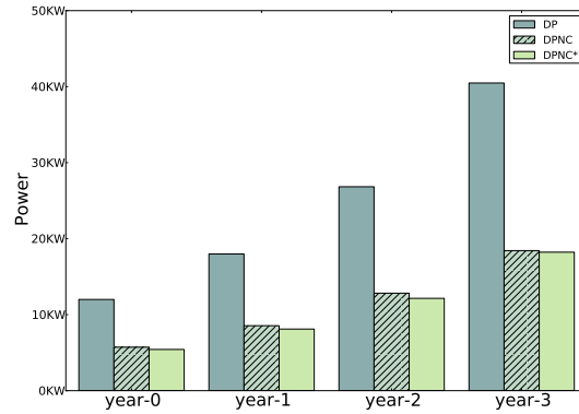
Figure 5. Overall Power Consumption of IP/MPLS line Cards.
