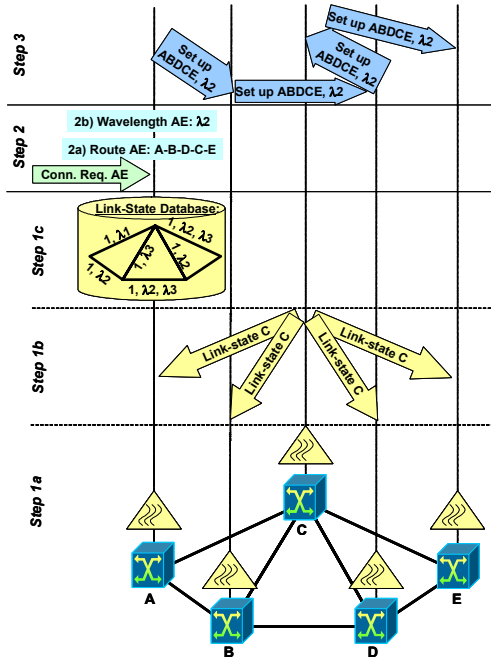
Figure 1. Principle of source-based link-state routing: 1a) each node filters link-state updates; 1b) flood link-state packets; 1c) each node constructs LSDB; 2) RWA; 3) Signal the set-up of the connection
