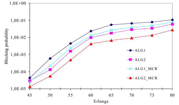
Figure 5. Effects of the MCR on the blocking probability when applied to ALG1 and ALG2
