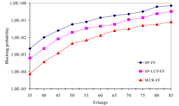
Figure 3. Blocking probability
