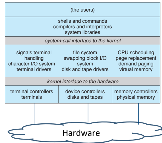
Fig. 2. UNIX System 1
